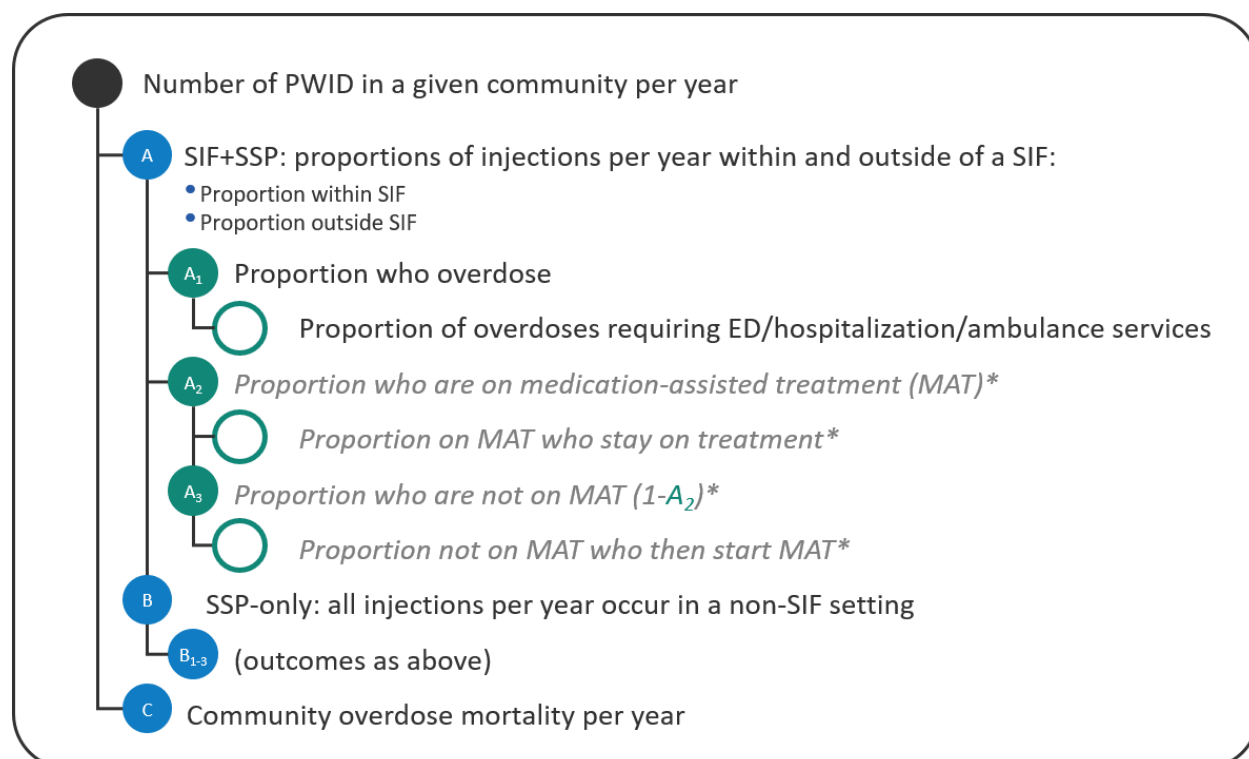
Figure 5.1. Model Framework
